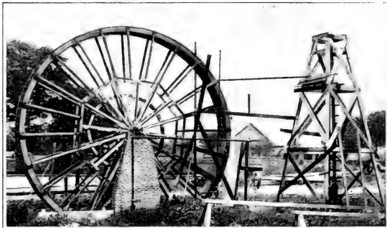
Electric current enough is generated by this plant, run by an artesian well, to operate a farm-mill, feed-chopper, lathe and other machinery used on the farm
